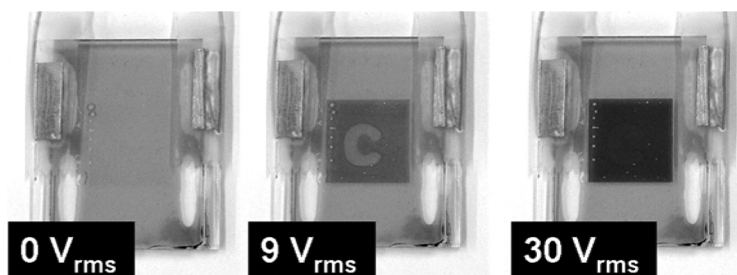
FIGURE 7 A multi-switch of the 5\text{-}\mu\text{m} gradient dye-doped LC gels at 0\text{ V}_{\text{rms}} , 9\text{ V}_{\text{rms}} and 30\text{ V}_{\text{rms}} .
