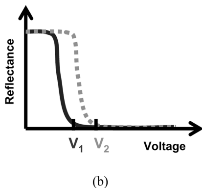
FIGURE 4 Schematic structure of gradient dye-doped LC gels (a) at voltage-off state and voltage-on state. (b) The corresponding voltage-dependent reflectance at the low density of polymer networks (solid line) and the high density of polymer networks (dotted line).
